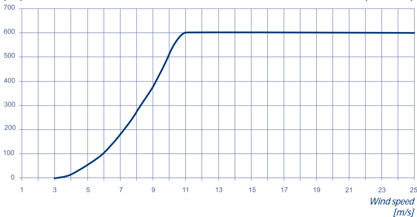
Power curve FL 600 (measured)
